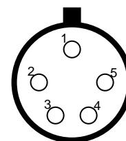
View onto solder buckets
