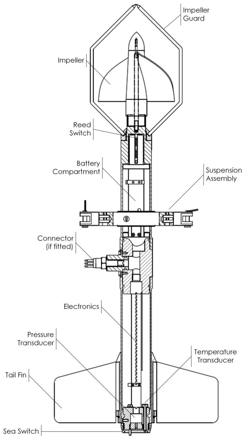
Figure 1: Model 106 Sensor Layout
