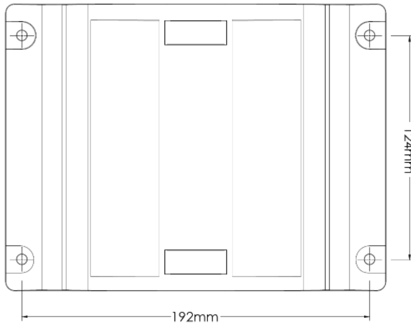
Figure 2 – TideMaster mounting template
