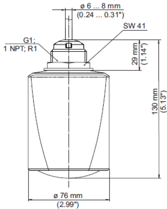
Figure 3 - VEGAPULS C23 dimensions
