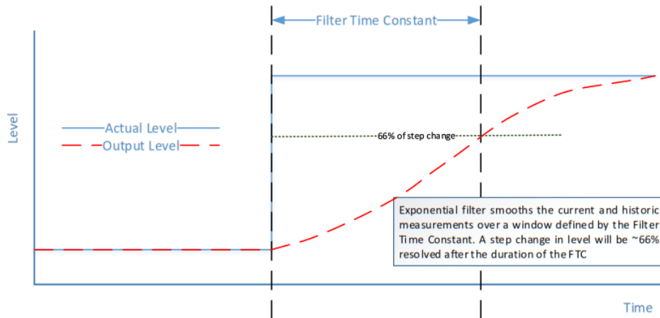
Exponential Filter
